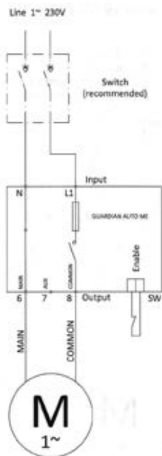
FIG. 4b: 2-WIRE MOTOR/PUMP
